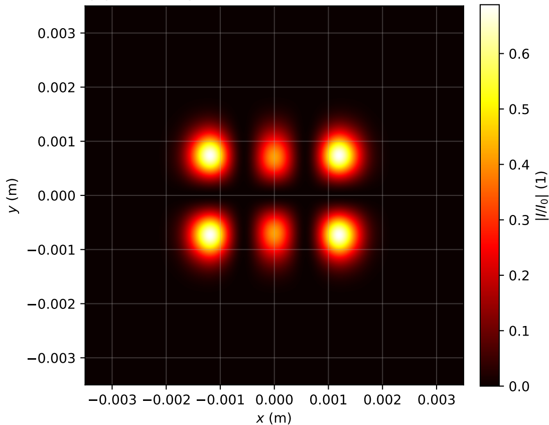
Intensity profile I(x, y, z = 2.229)/I_0 , P_{in}=2.0P_{cr} , artificial time
